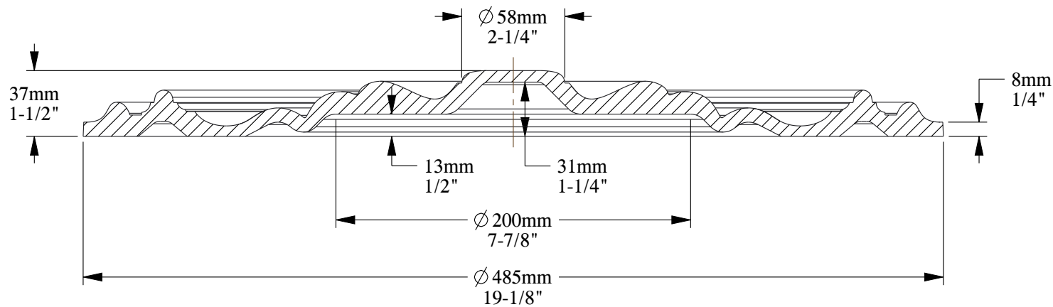
SECTION A-A SCALE 33:100
